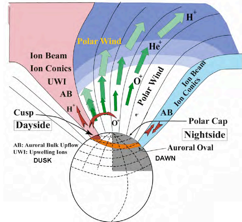
Figure 9 Polar Wind outflows (source: www.semanticscholar.org )
