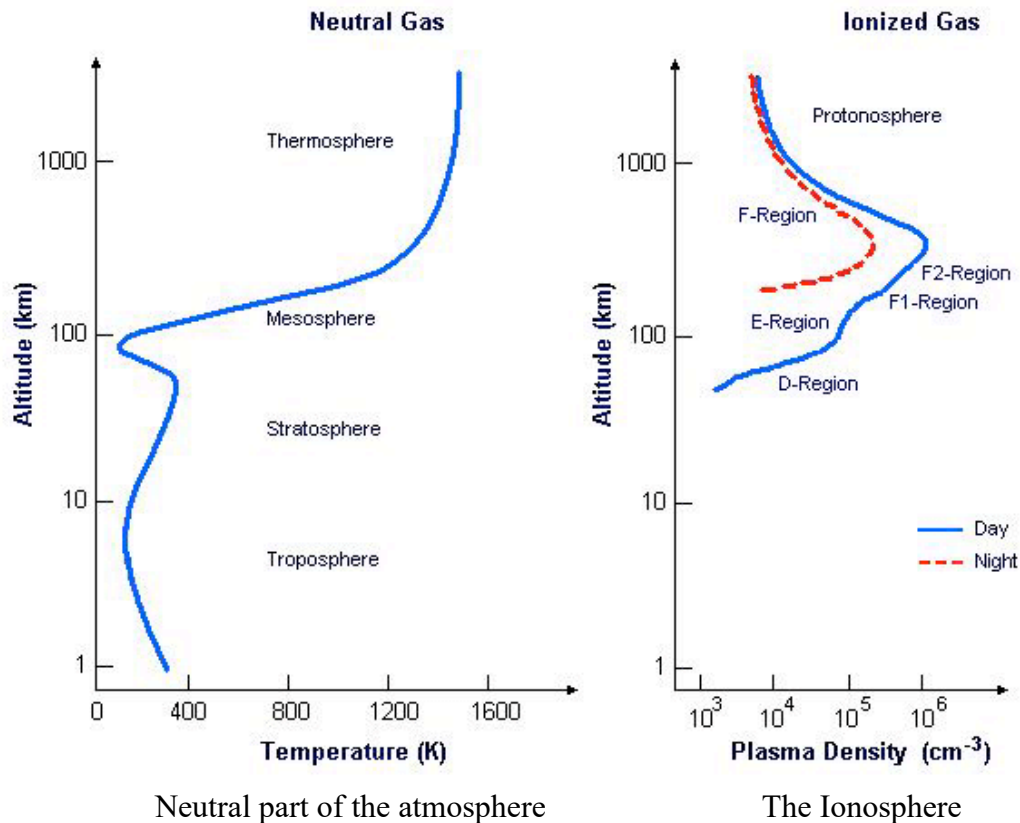
Figure 16 Structure of Earth’s atmosphere and ionosphere (source: ResearchGate)
