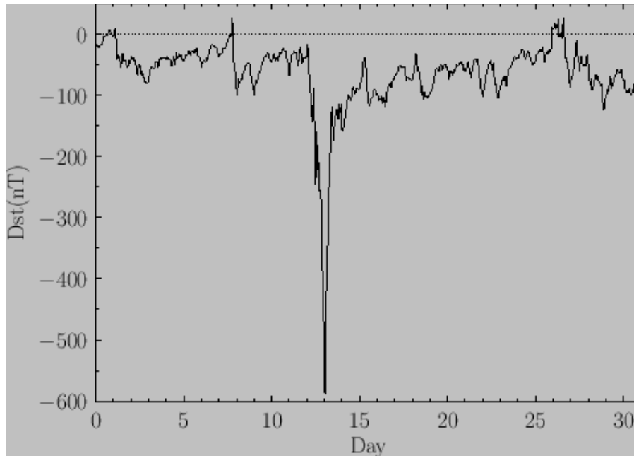
Figure 23 Dst index for the month of March 1989 (source: Farside.ph.utexas.edu)
