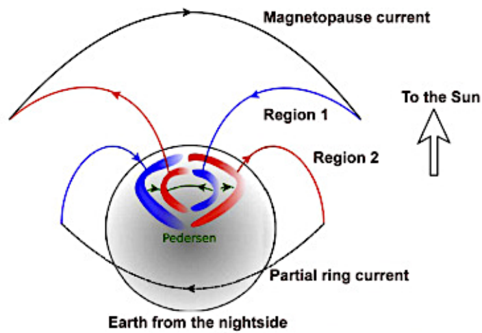
Figure 31 Region 1 and Region FAC (source: ScienceDirect.com)
