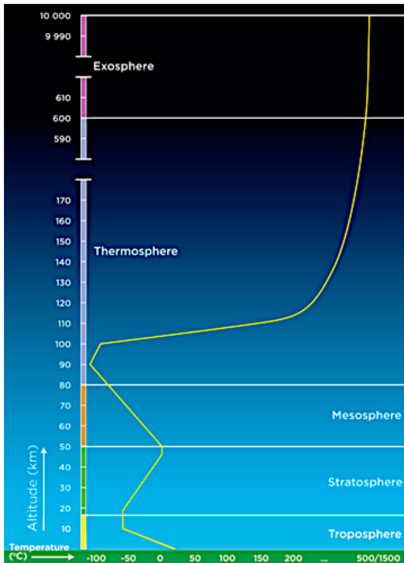
Figure 15 Layers of Earth’s atmosphere (source: siyavula.com)
