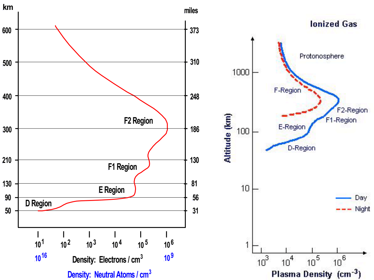
Figure 8 Electron density of Earth's ionosphere (source: author)
