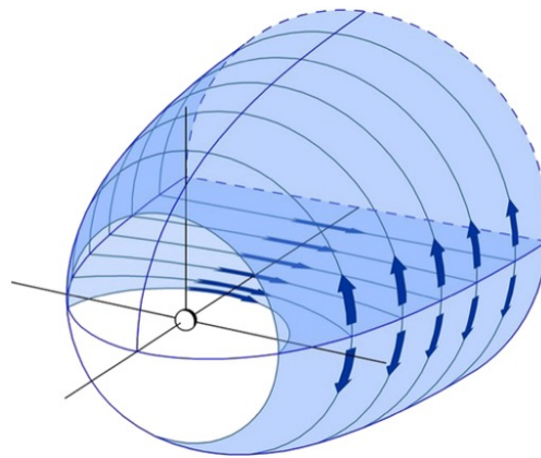
Figure 27 Magnetosphere cross-tail electrical current (source: Ganushkina et al)
