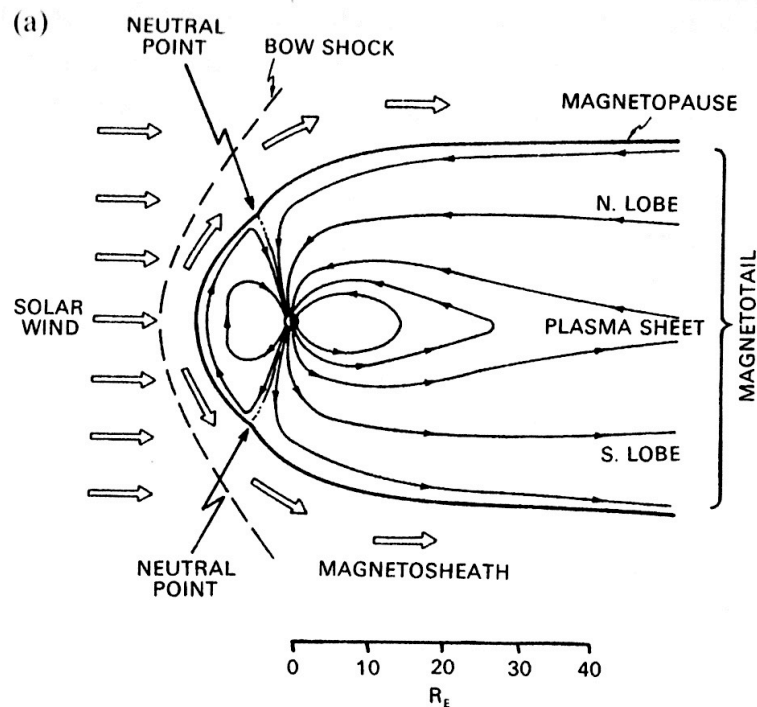
Figure 4 Magnetotail (source: Hunsucker)
