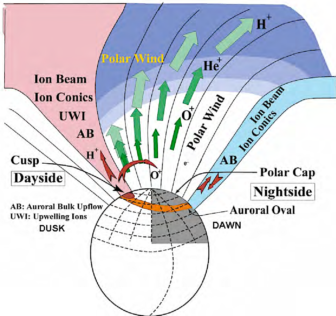
Figure 6 Polar Wind outflow (source: www.semanticscholar.org )
