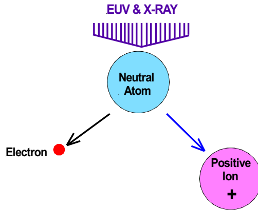
Figure 7 Photoionization process (source: author)
