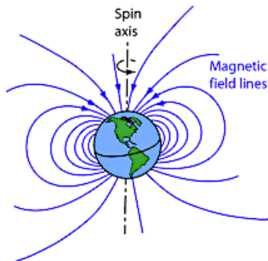
Figure 1 Earth's dipolar magnetic field (source: Hyperphysics)
