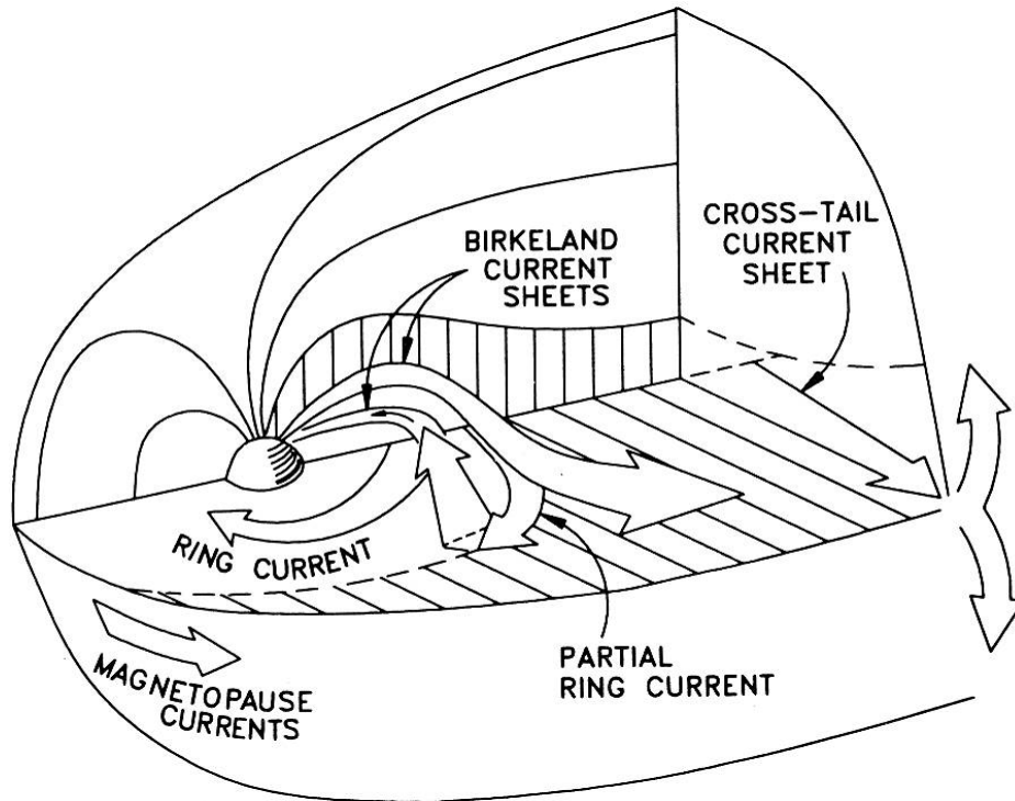
Figure 24 Magnetosphere Electrical Currents (source: Wikipedia)
