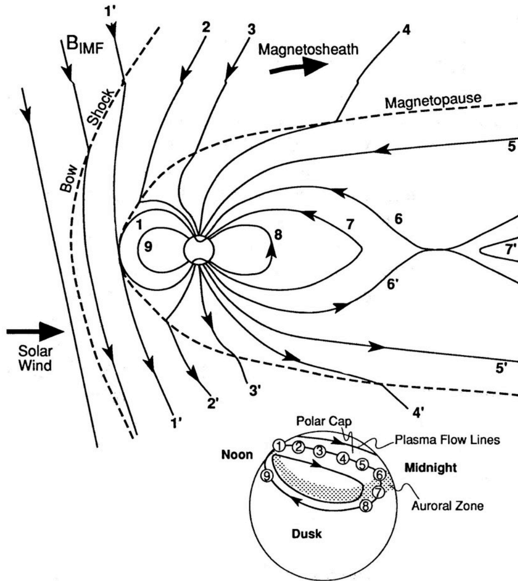
Figure 34 Dungey convection cycle (source: ResearchGate)
