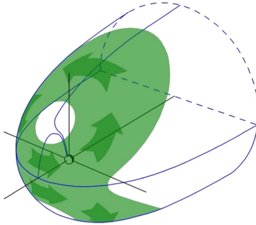
Figure 25 Chapman-Ferraro magnetopause electrical current (source: Ganushkina et al)
