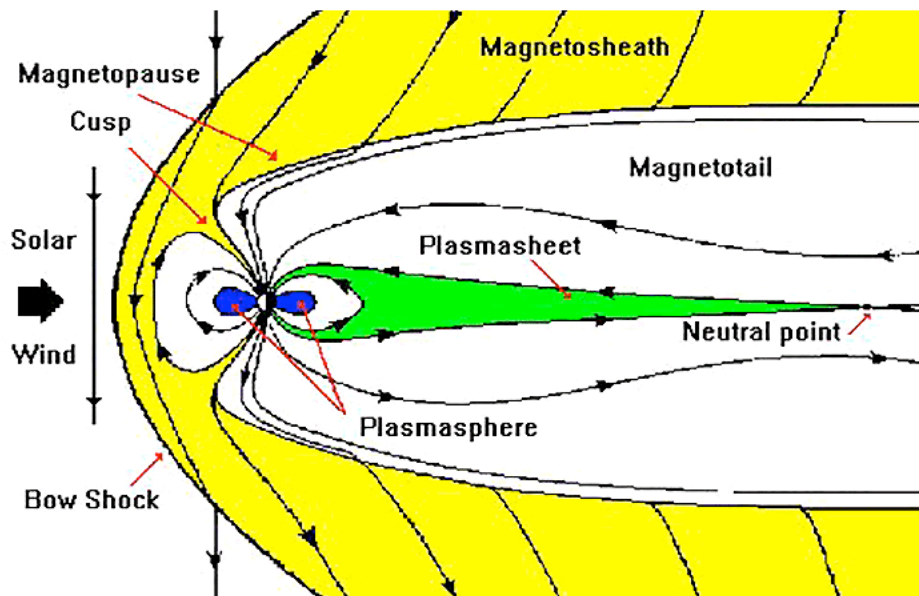
Figure 18 Plasmasheet (source: ResearchGate)
