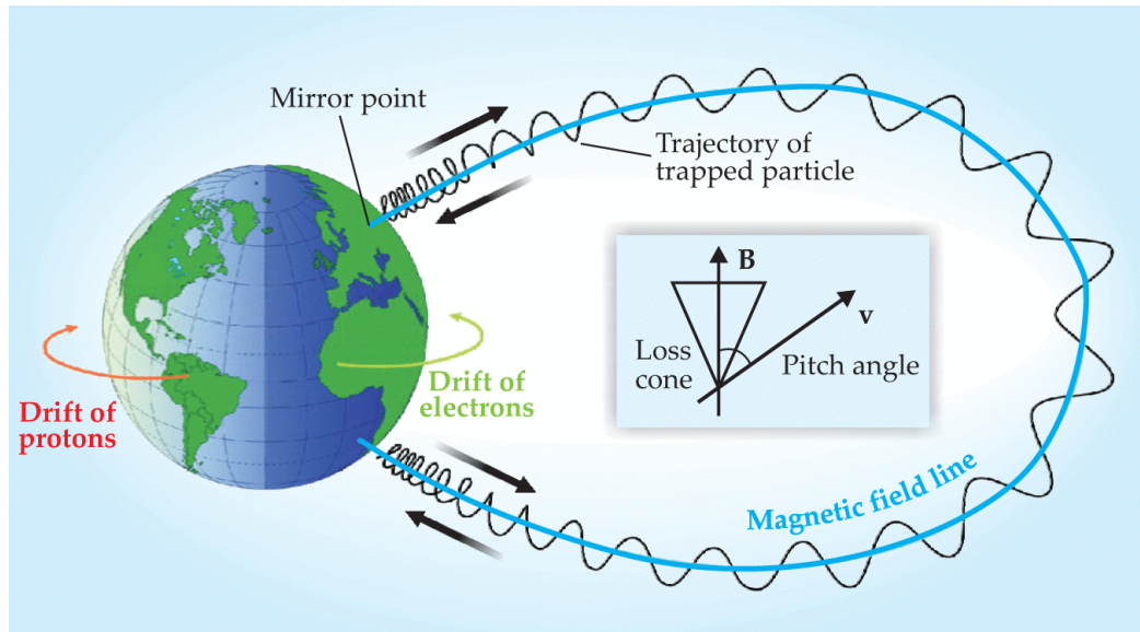
Figure 19 Trapped Charged Particles (source: Physics Today – Scitation)
