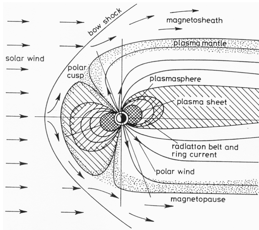
Figure 5 Earth's Magnetosphere (source: Davies)
