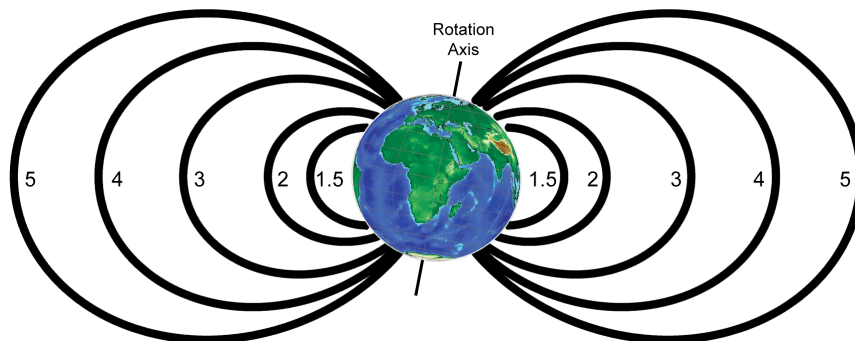
Figure 21 Various L – shells (source: Wikipedia)
