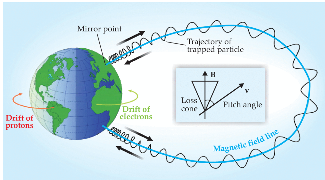
Figure 22 Formation of Ring Currents (source: Physics Today – Scitation)
