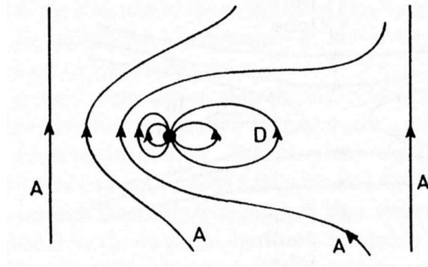
Figure 35 North Directed IMF (source Hunsucker)
