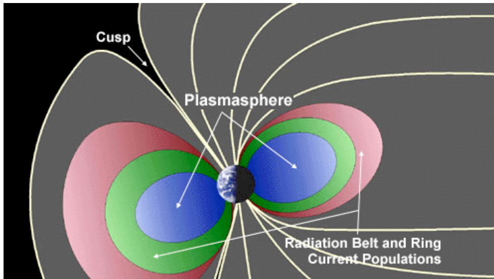
Figure 14 Plasmasphere (source: Alchetron)
