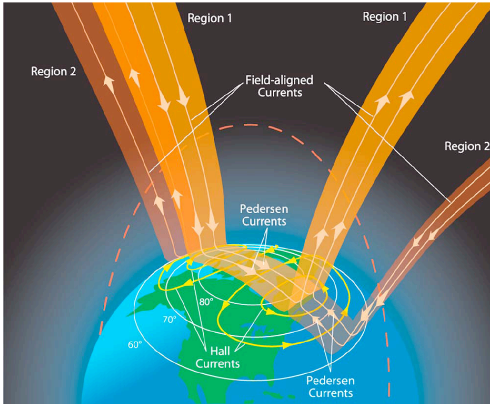
Figure 30 Field Aligned Currents (source: Wikipedia)
