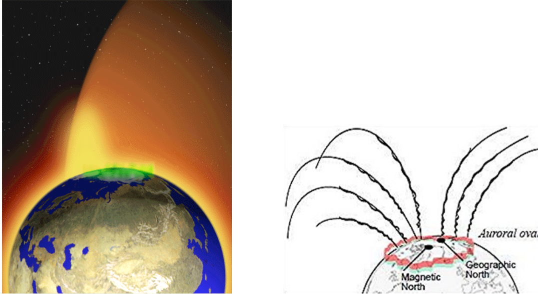
Figure 10 Ion fountain (source: Wikipedia)
