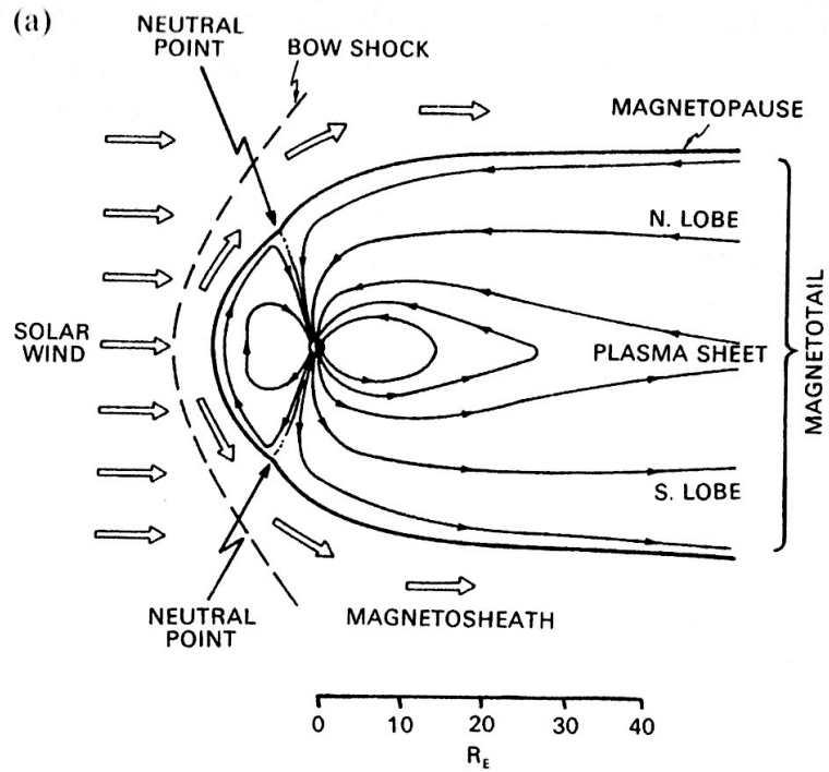
Figure 26 Magnetotail (source: Hunsucker)
