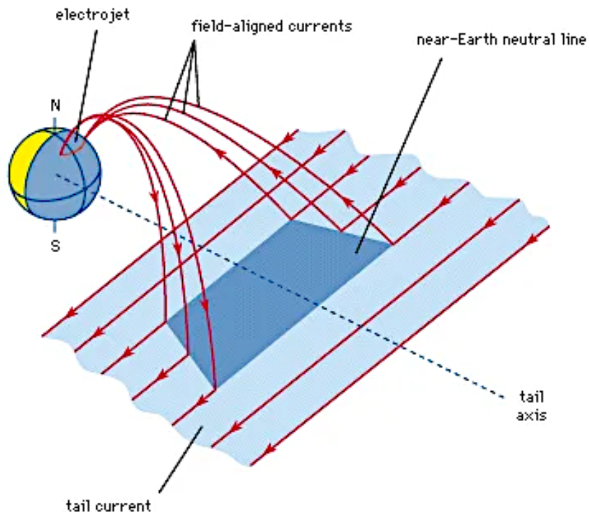
Figure 29 Magnetotail current wedge (source: Encyclopaedia Britannica)
