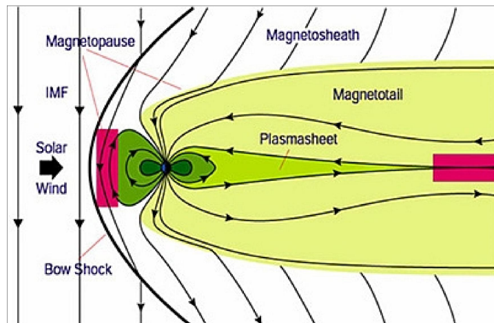
Figure 33 Magnetic neutral points (source: Satellite Missions)
