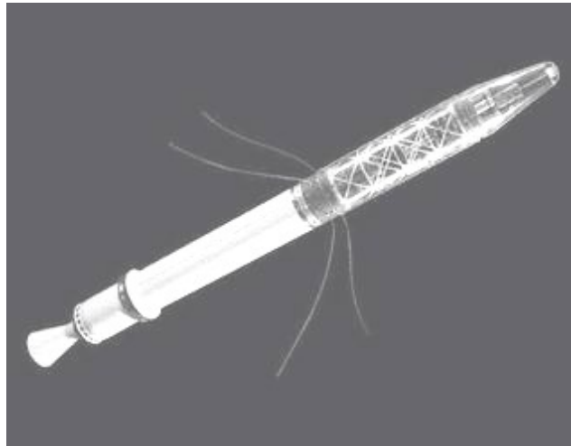
Figure 12 Explorer 1 Satellite (source: NASA)
