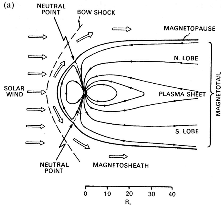
Figure 17 Magnetotail (source: Hunsucker)
