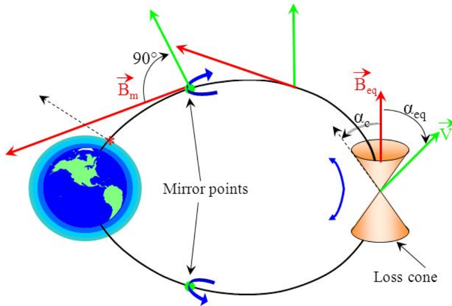
Figure 20 Loss Cone (source: Slideplayer.com)
