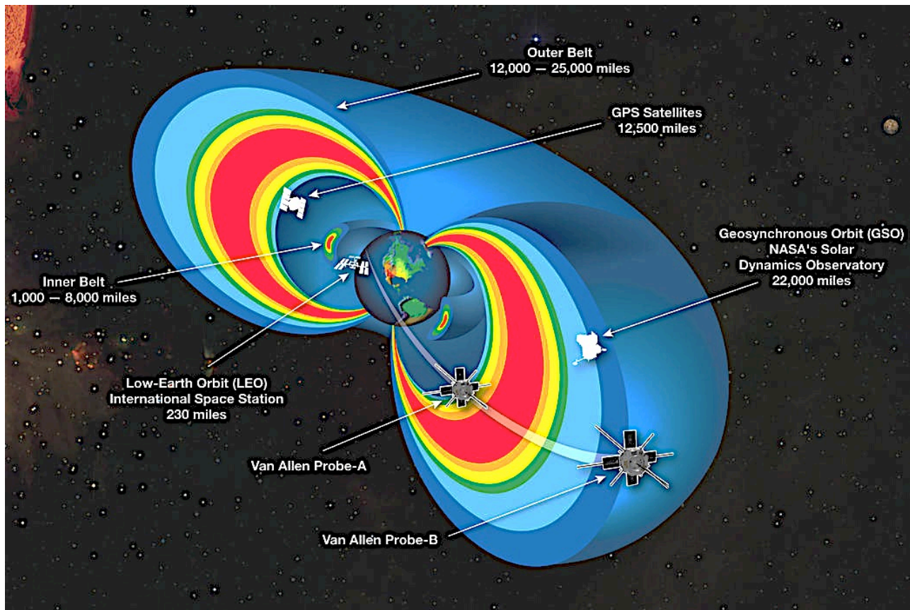
Figure 11 Cutaway model of the radiation belts (source: NASA)
