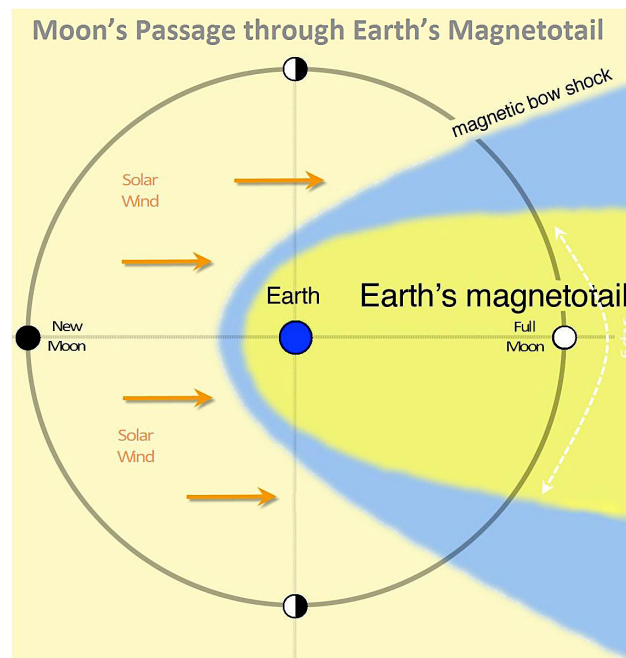
Figure 3 Earth's magnetic field tail stretches out past the moon (source: Time-Price-Research)
